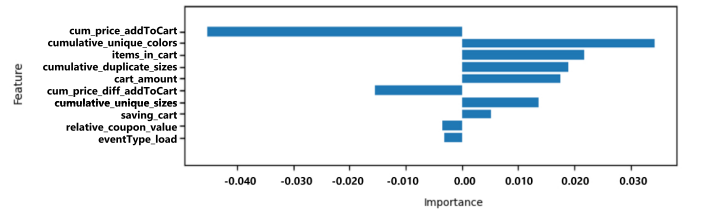
Fig. 6. Top 10 features for desktop users with \hat{\beta}_u = 1 .
