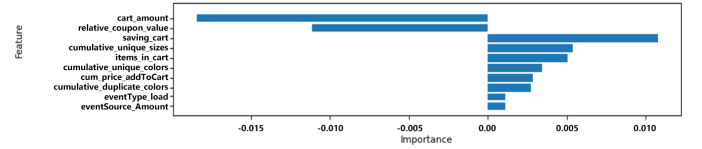
Fig. 5. Top 10 features for mobile users with \hat{\alpha}_u = 1 .
