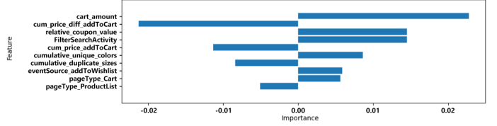
Fig. 4. Top 10 features for desktop users with \hat{\alpha}_u = 1 .
