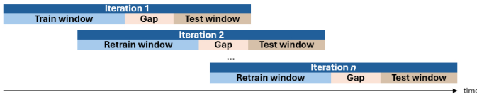
Fig. 3. Generalized framework of our train-test setting.
