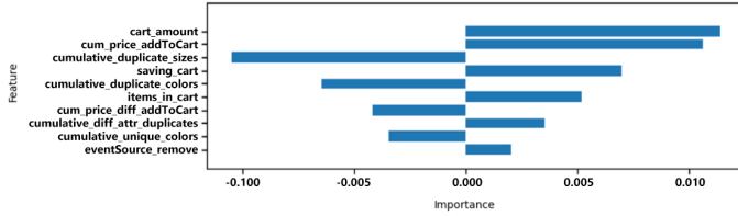
Fig. 8. Top 10 features for desktop users with \hat{\gamma}_u \in (0.6, 0.9] .
